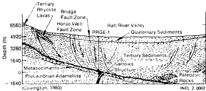
Figure 2. Cross-sectional view of major structures across the Raft River KGRA.
