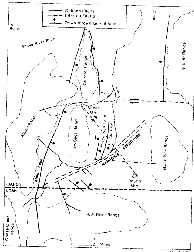
Figure 1. Major structural features of the southern Raft River Valley.
