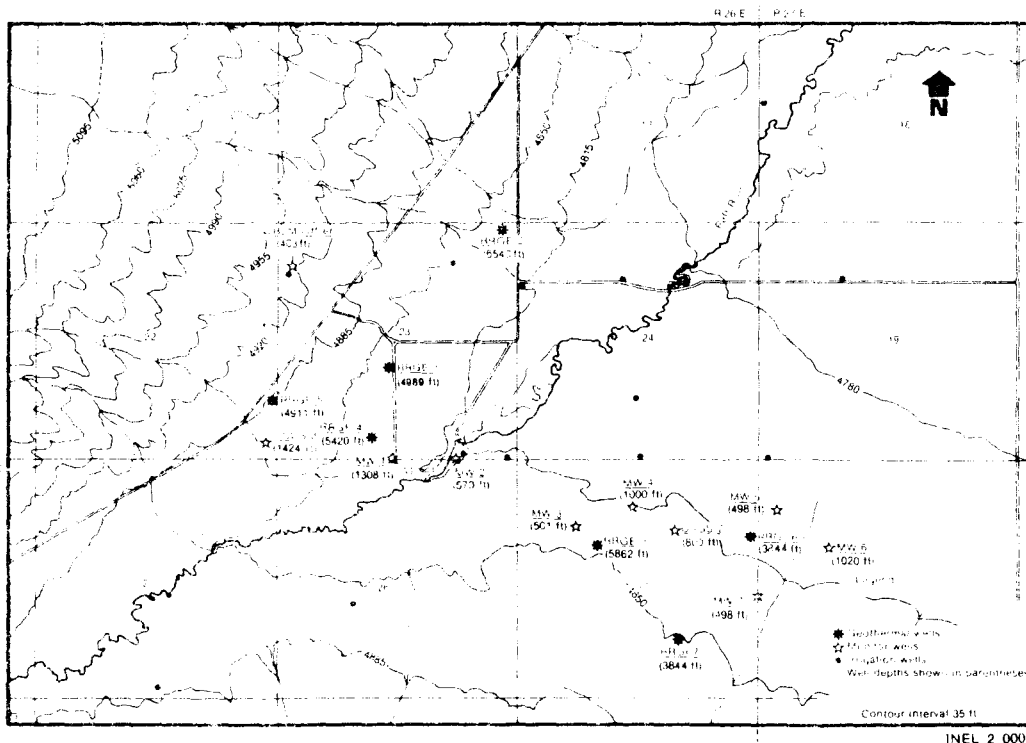
Figure 3. Raft River Well Field.
