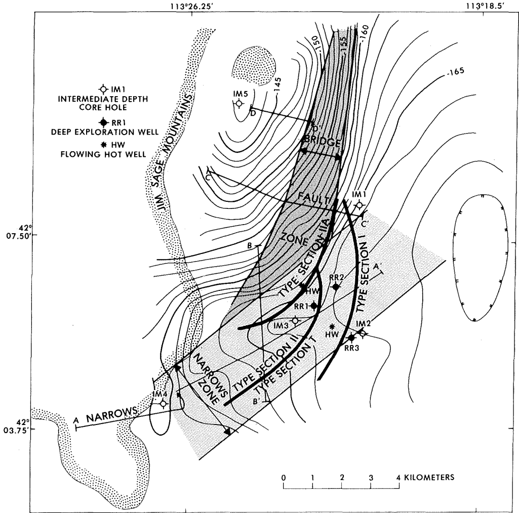
FIG. 3. Map showing locations of velocity sections A-A', B-B', C-C', and D-D', the boundaries of type sections I, T, II and IIA, the exploration and flowing hot wells, the Bridge fault zone, and the inferred Narrows zone and Bouguer gravity anomaly contours (Mabey et al, 1978).
