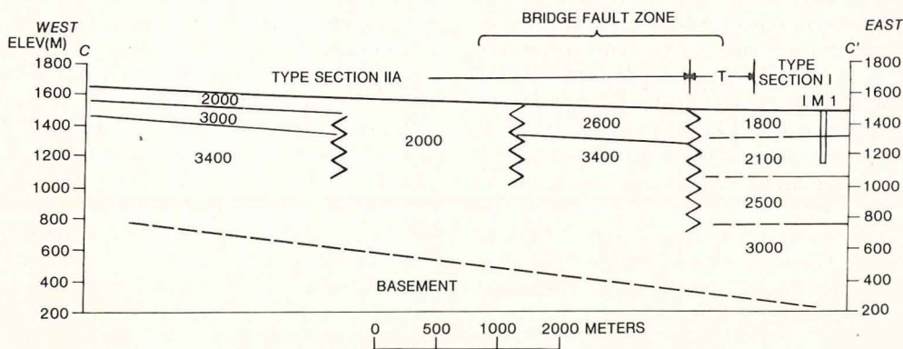
FIG. 5. Velocity section C-C'. Velocities are in m/sec and the vertical exaggeration is 1.3 times.
