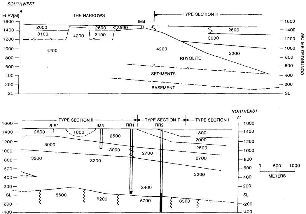
FIG. 2. Velocity section A-A' interpreted from spreads along the Raft River. Velocities are in m/sec. Vertical exaggeration is 1.3 times. Location of A-A' is shown in Figure 3.
