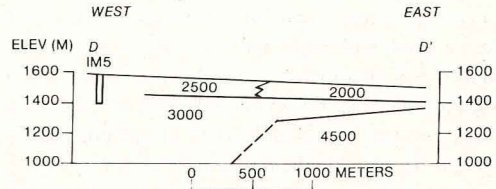
FIG. 6. Velocity section D-D'. Velocities are in m/sec and the vertical exaggeration is 1.3 times.
