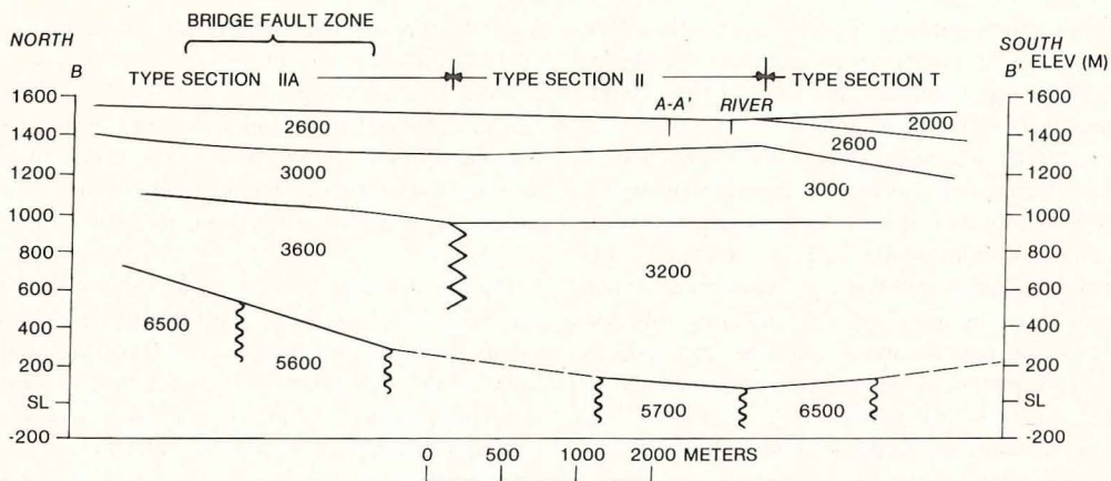
FIG. 4. Velocity sections B-B'. Velocities are in m/sec and the vertical exaggeration is 1.3 times.
