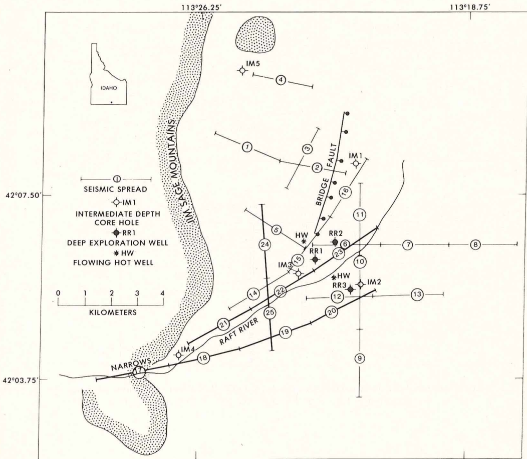
FIG. 1. Location of seismic spreads, exploration wells, and flowing hot wells in the Raft River geothermal area. Spreads with complete reverse coverage of the basement horizon are shown with heavy lines.
