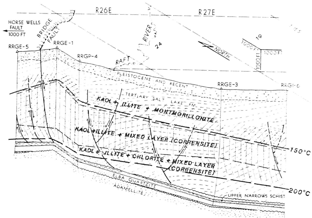
Figure 4: Generalized zonation of clay minerals within the Raft River geothermal system.
