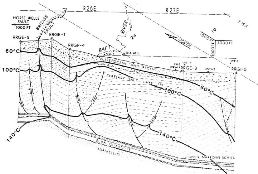
Figure 3: Isometric diagram showing subsurface geology and temperature distribution within the Raft River geothermal system.
