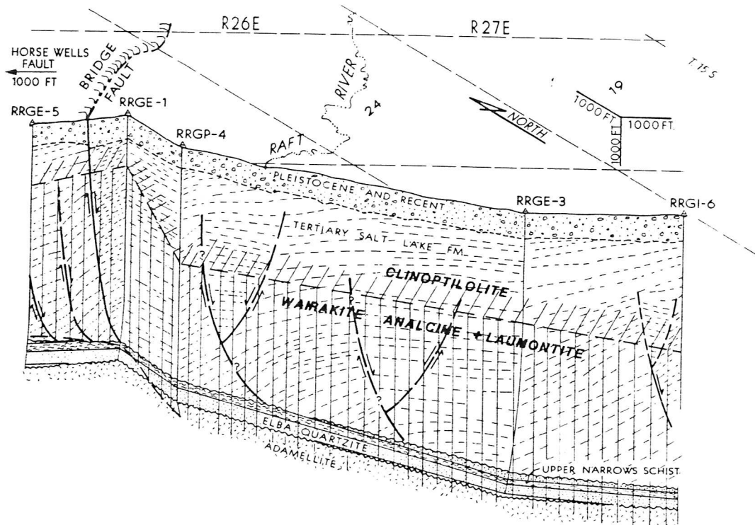
Figure 5: Generalized zonation of natural zeolites within the Raft River geothermal system.
