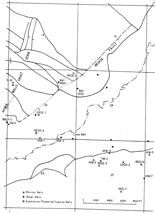
Figure 2: Raft River Well Field Diagram
