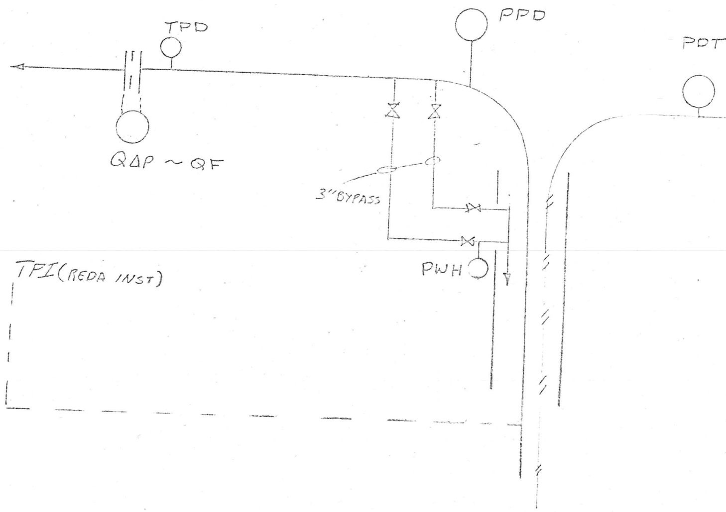
RRGF WELL #1 INSTRUMENTATION LOCATIONS
