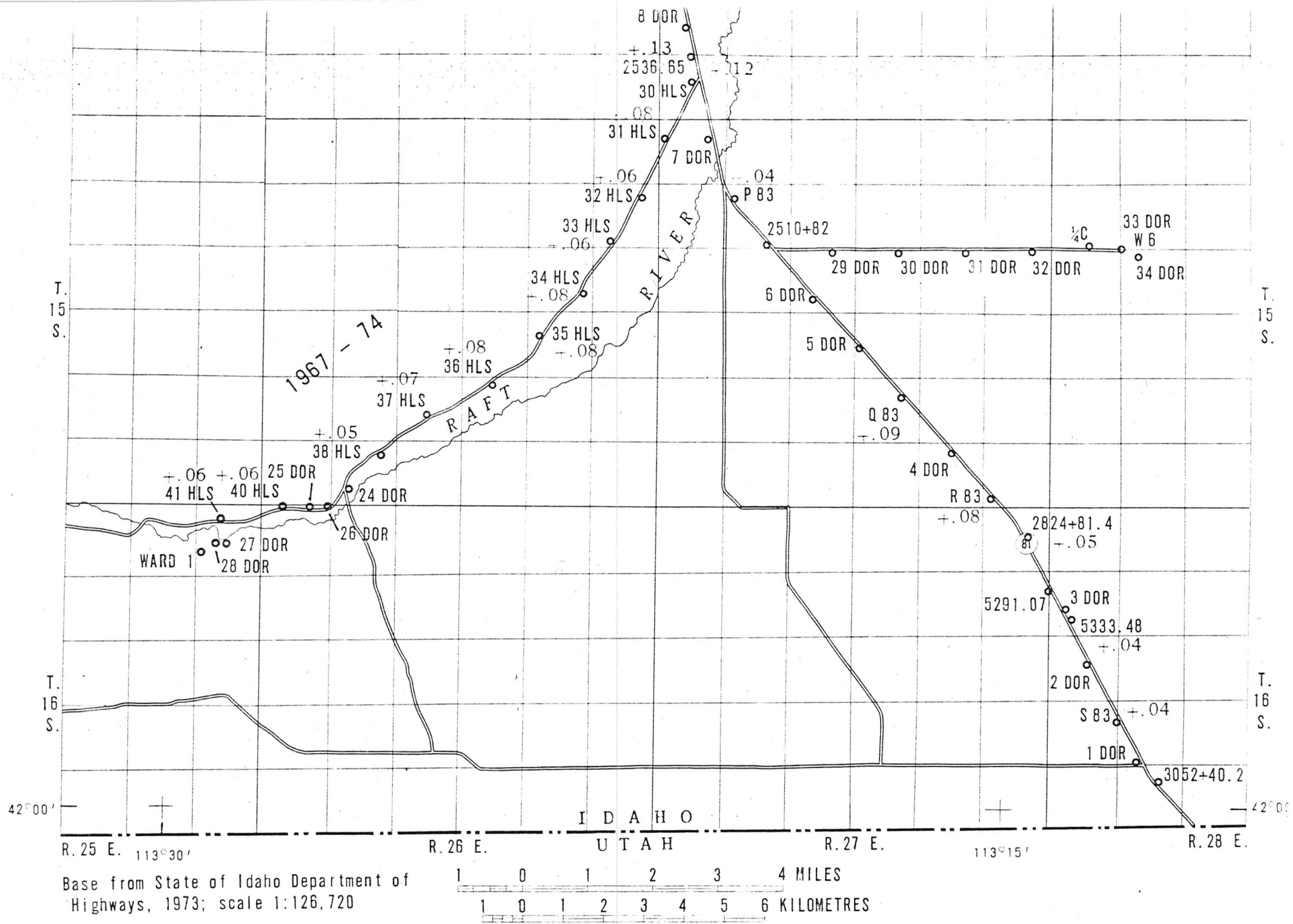
FIGURE 2.—Measured change in elevation of bench marks, Raft River Valley, Idaho
